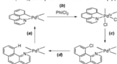
Scheme 1. Pd(OAc) 2 -Catalyzed Chlorination of Benzo[ h ]quinoline a
